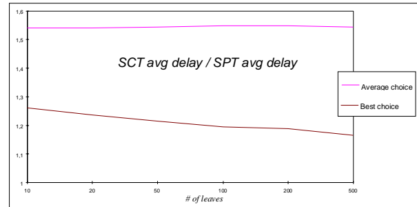
Figure 8 : SCT et SPT average delays
