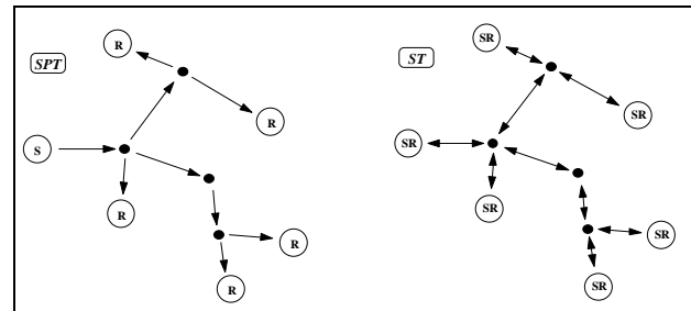
Figure 5 : Shortest Path and Shared Trees
